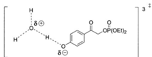
Figure 5. Suggested transition state for the rate determining adiabatic triplet state proton transfer to H_2O .
