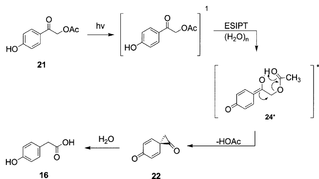
Figure 2. ES IPT singlet state photorelease mechanism of the p -hydroxyphenacyl acetate [7].
