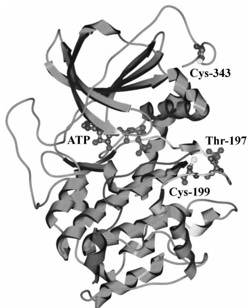
Figure 13. Protein Kinase: Thr 197 and Cys-199 are shown at the active site [28]. Reprinted with permission from ref. 29 © American Chemical Society.
