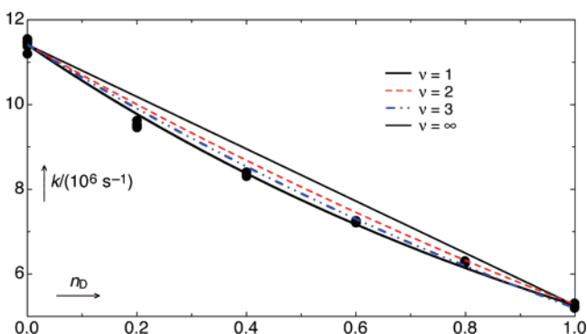
Figure 4. Decay rate constants k_n of T 1 ( 1a ) in degassed 10% (by vol) aqueous CH 3 CN at 25 ± 0.1 °C at various atom fractions of deuterium n in the aqueous part of the solvent. The upper solid line shows the expectation (eq 2, \nu = 1 ) for a single-site isotope effect of 2.17, and the lower solid line shows the expectation (eq 3) for a generalized solvation effect from many sites. The intermediate dashed lines correspond to a two-site effect (red, isotope effect of 1.5 at each site; eq 2, \nu = 2 ) and a three-site effect (blue, isotope effect of 1.3 at each site; eq 2, \nu = 3 ).
