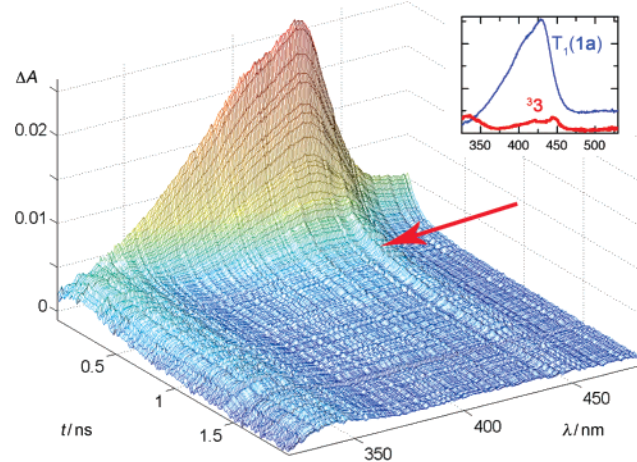
Figure 1. Pump-probe spectroscopy of 1a in 87% aqueous CH 3 CN. The sample was excited with a pulse from a Ti:Sa-NOPA laser system (266 nm, 150 fs pulse width, pulse energy 1 μJ). 10 The inset shows the species spectra of T 1 and 3 3 that were determined by global analysis of the spectra taken with delays of 10–1800 ps using a biexponential fit.
